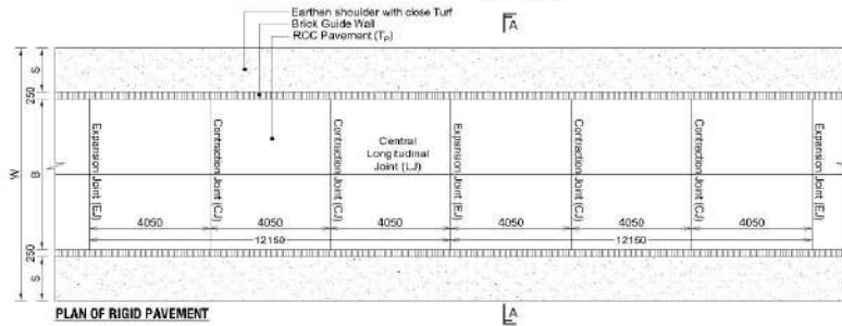
PLAN OF RIGID PAVEMENT
