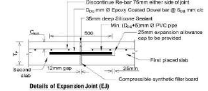
Details of Expansion Joint (EJ)
