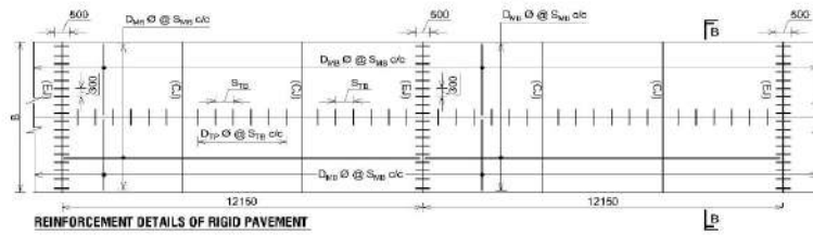
REINFORCEMENT DETAILS OF RIGID PAVEMENT
